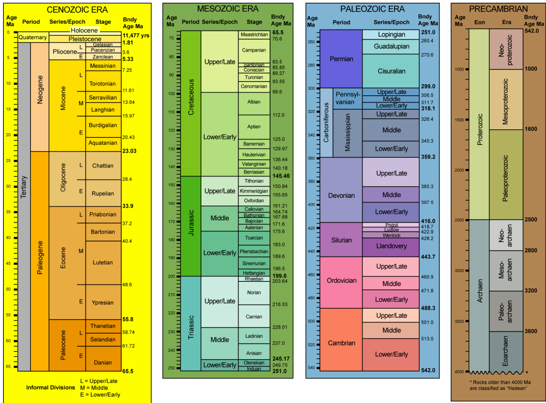
Figure 2. Geologic Time Scale. Ma = Millions of years old. Bndy Age = Boundary Age. Colors are USGS standard colors found on geologic maps. Modified from 1999 Geological Society of America Time scale ( www.geosociety.org/science/timescale/timescl.pdf ). Boundary dates and additional information from 2004 International Commission on Stratigraphy ( www.stratigraphy.org/gssp.htm ) and U.S. Geological Survey Fact Sheet 2007-3015 ( http://pubs.usgs.gov/fs/2007/3015/ ).
