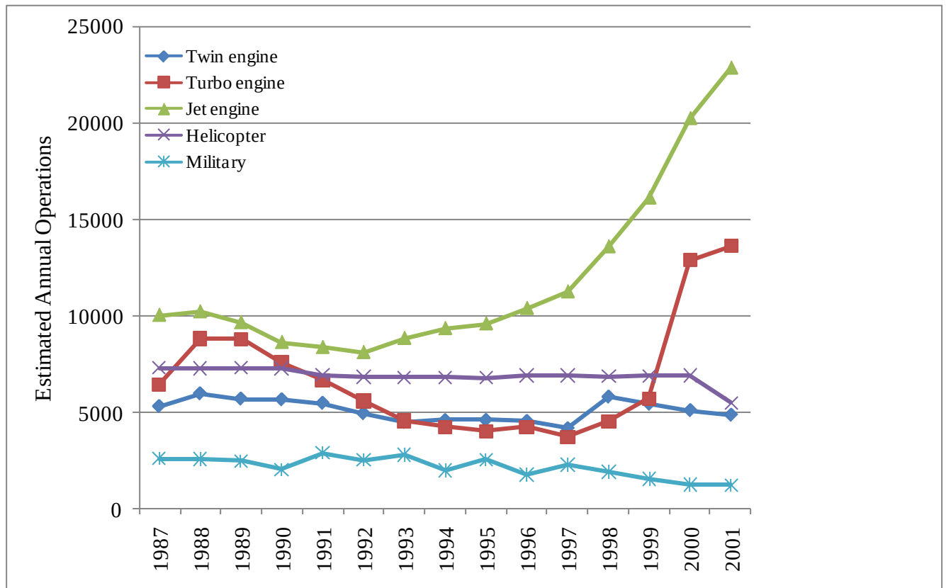
Figure 28. Estimated annual operations for selected aircraft at L.G. Hanscom Field from 1987 to 2001 (Data from Arnold 2002).
