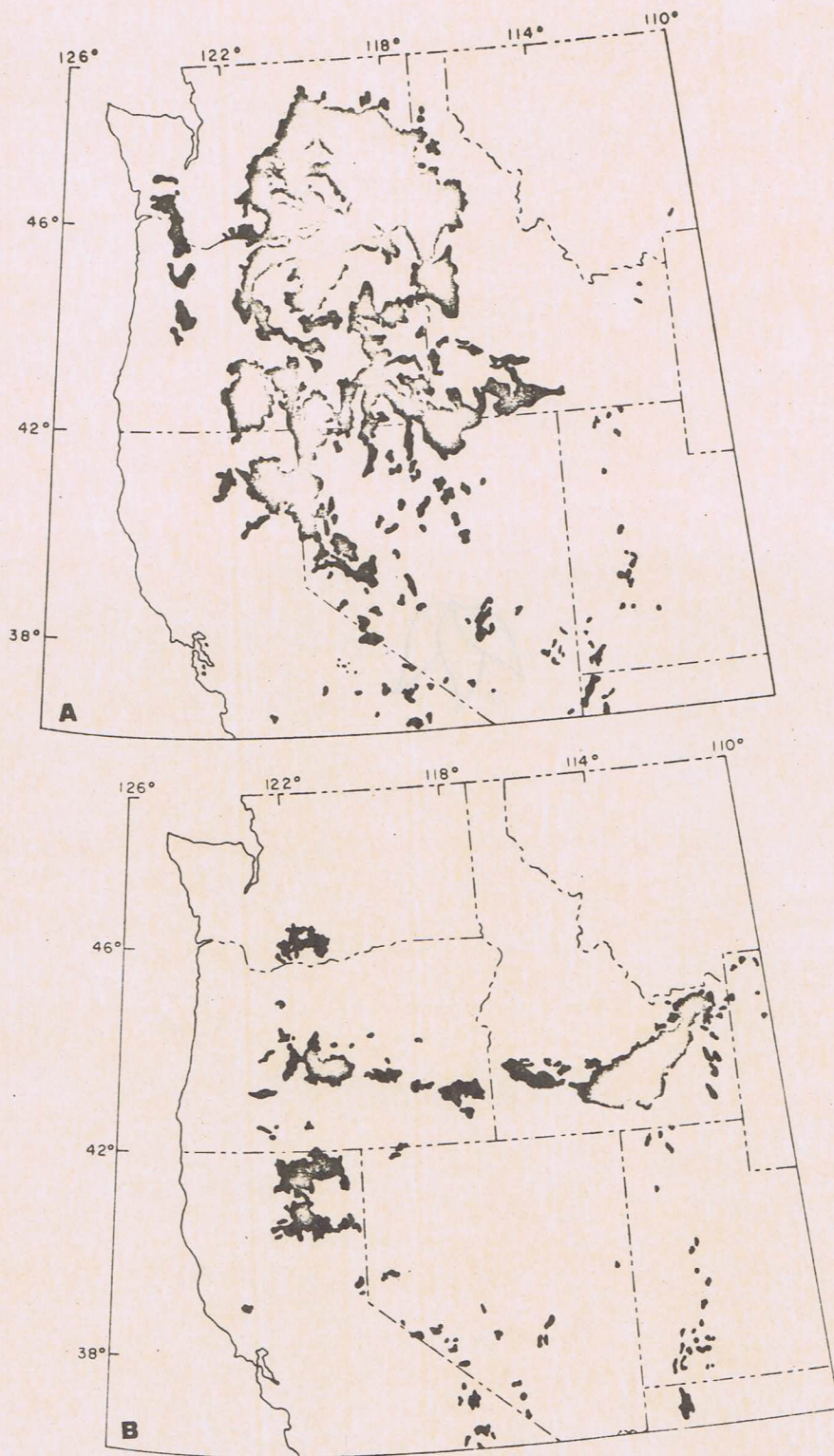
Figure 13-4. Maps showing distribution of Tertiary and Quaternary basalt in the Great Basin and Columbia Intermontane regions. (A) Tertiary basalts less than 17 m.y. old. (B) Quaternary basalts. (In part after Stewart and Carlson, 1976.)
