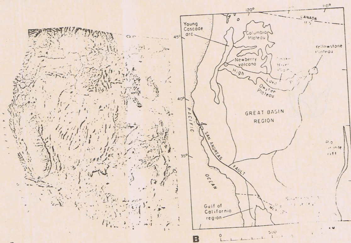
A B Figure 13-1. Physiography of the Western United States. (A) Shaded relief map; note well-defined physiographic break between the northern and southern parts of the Basin and Range province (after U.S. Geol. Survey, National Atlas of the United States of America , p. 56). (B) Index to some late Cenozoic tectonic and volcanic features shown on Figure 13-1A.
