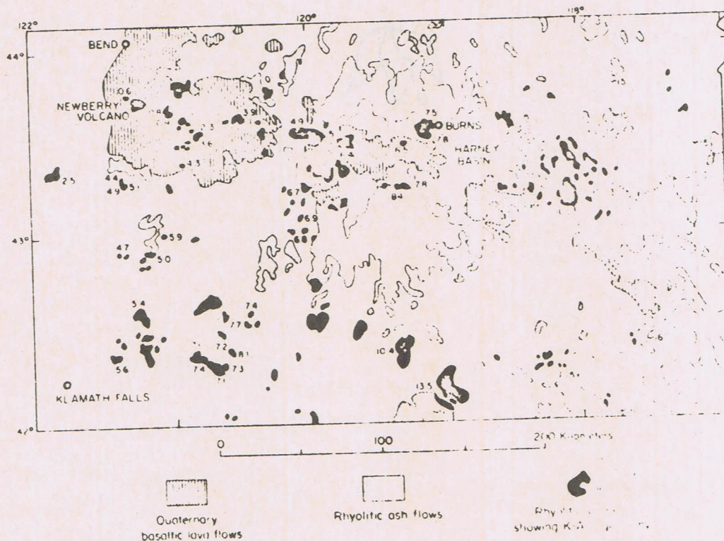
Figure 13-7. Map showing distribution of upper Cenozoic volcanic rocks in south-central Oregon. Rhyolite domes and ash-flow tuffs decrease in age from about 17 m.y. in the southeast to less than 1 m.y. in the northwest. (After MacLeod and others, 1976.)
