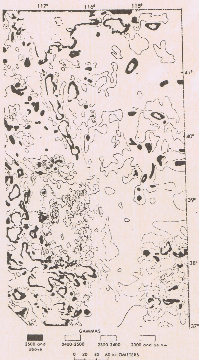
Figure 13-5. Aeromagnetic map of central and northeastern Nevada. Note the similarity between the outcrop pattern of basalts (Fig. 13-4) and many of the aeromagnetic highs, especially the north-trending belt in the central to northern part of the state. (After Stewart and others, 1977.)
