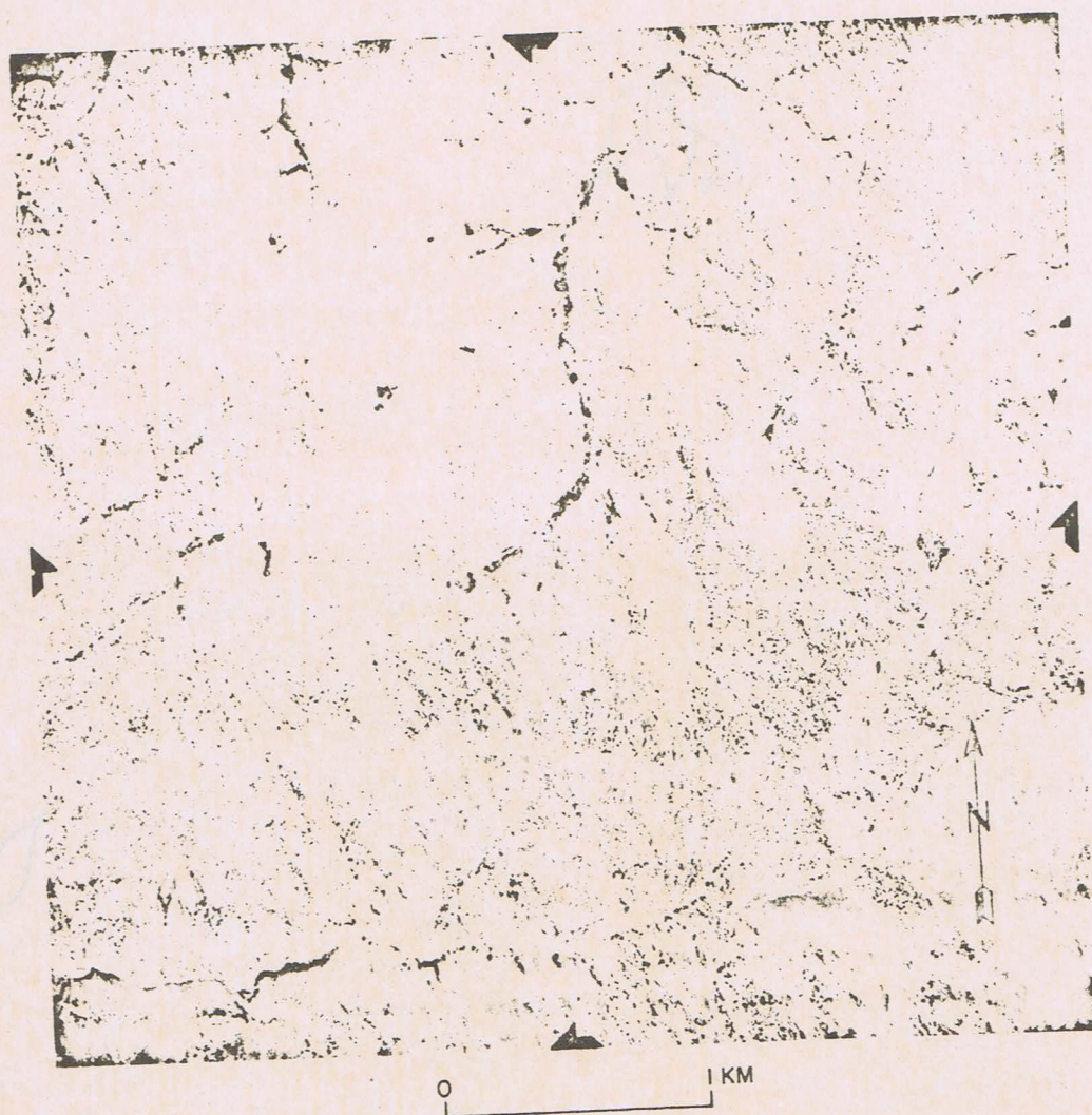
Figure 13-6. Aerial photograph of basaltic dike swarm in the western part of the Roberts Creek Mountains, near the southern end of the linear aeromagnetic high of central Nevada (Fig. 13-5). Lines trending north-northwest across topographic features are nearly vertical dikes.
