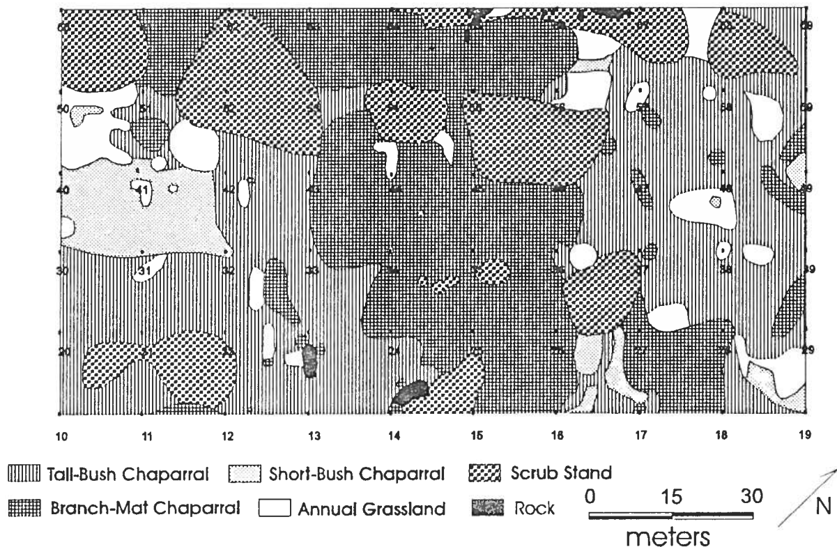
Figure 5. Traugers Plot showing the trapping grid and the boundaries of major vegetation types. The steel stakes that mark the stations are located directly above the station numbers.
