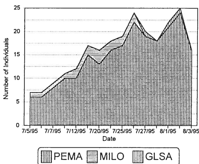
Figure 4. Daily modified Jolly-Seber estimates of the rodent population at the Atwell Plot.
