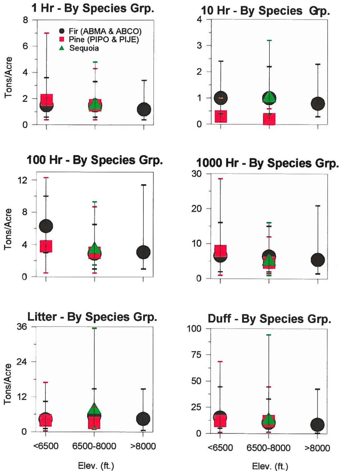
Figure 15. Summarized fuels data obtained from 1995 transects showing average and range of values for major fuel categories. Data have been divided into the three main vegetation types for the watershed and into three broad elevational zones.
