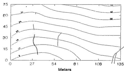
Figure 3. Atwell Plot showing topography in 5 m contour intervals and location of surface water.
