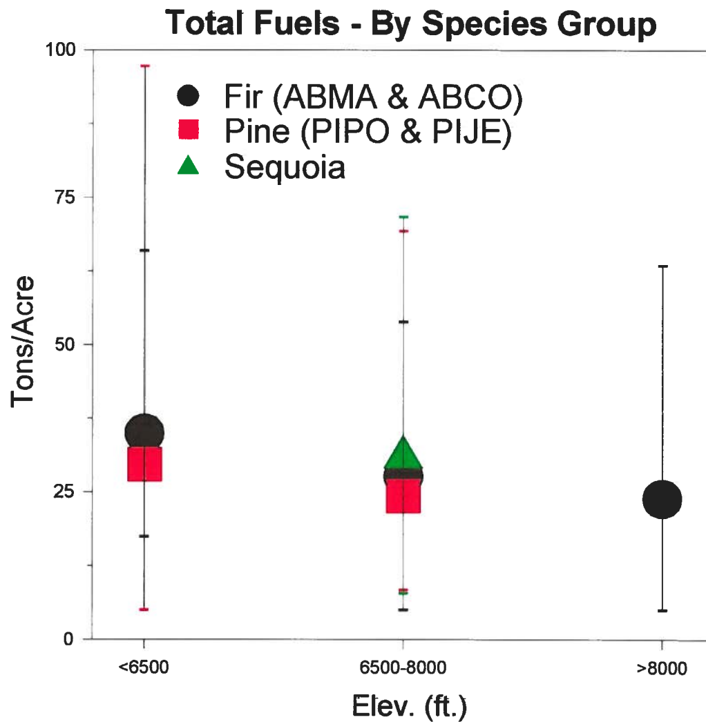
Figure 16. Summarized data for total fuels showing average and range of values. Data have been divided into the three main vegetation types for the watershed and into three broad elevational zones.
