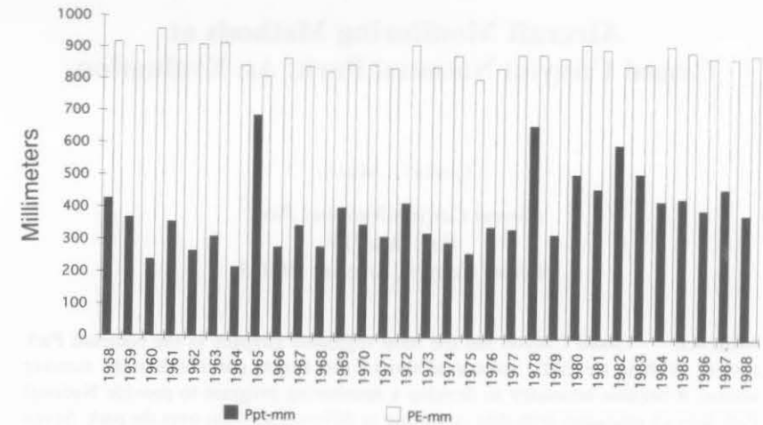
Fig. 4. Precipitation and potential evaporation near Beaver Creek.
