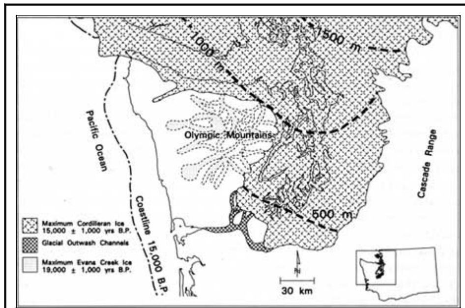
Fig. 3. The Olympic Peninsula, showing the distribution of glaciers during the Evans Creek stade and the extent of Cordilleran ice during the Vashon stade. The extent of Evans Creek glaciation is speculative and based on incomplete surveys. Modified from Crandell (1964, 1965), Moore (1965), Carson (1970), Heusser (1974), Waitt and Thorson (1983), and Booth (1987).
