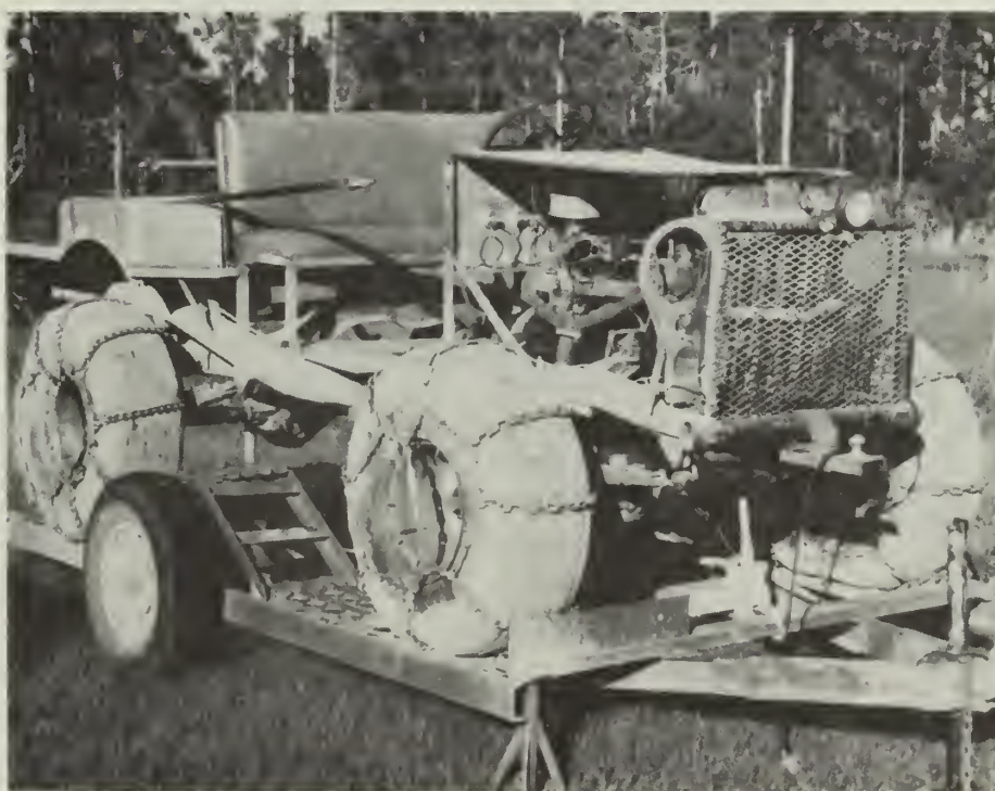
Figure 6. One of our "intermediate" swamp buggies. It was the "smooth" buggy without chains and the "chain" buggy with chains.
