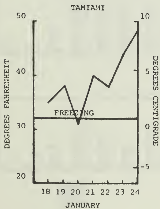
Figure 9: 1977 January Freeze in South Florida
