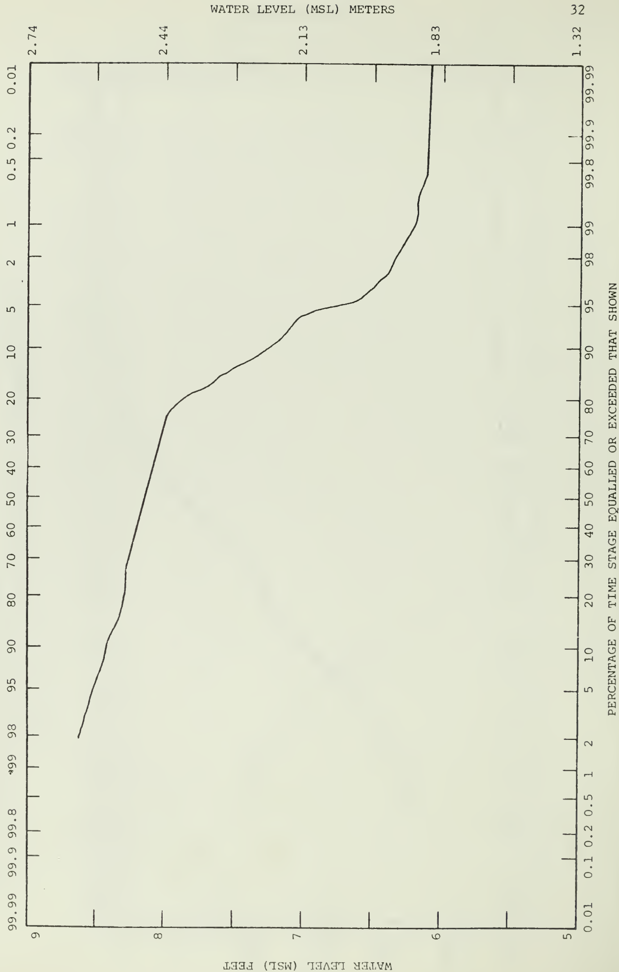
Figure 19: Stage Duration Curve for Tamiami Canal Outlets: At 40 Mile Bend, 1977
