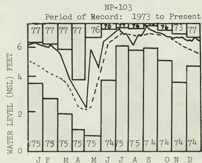
Figure 12: Big Cypress Hydrographs for 1977
