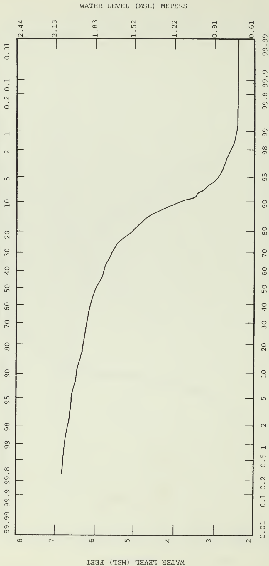
Figure 21: Stage Duration Curve at NP-103 (Pinecrest), 1977
