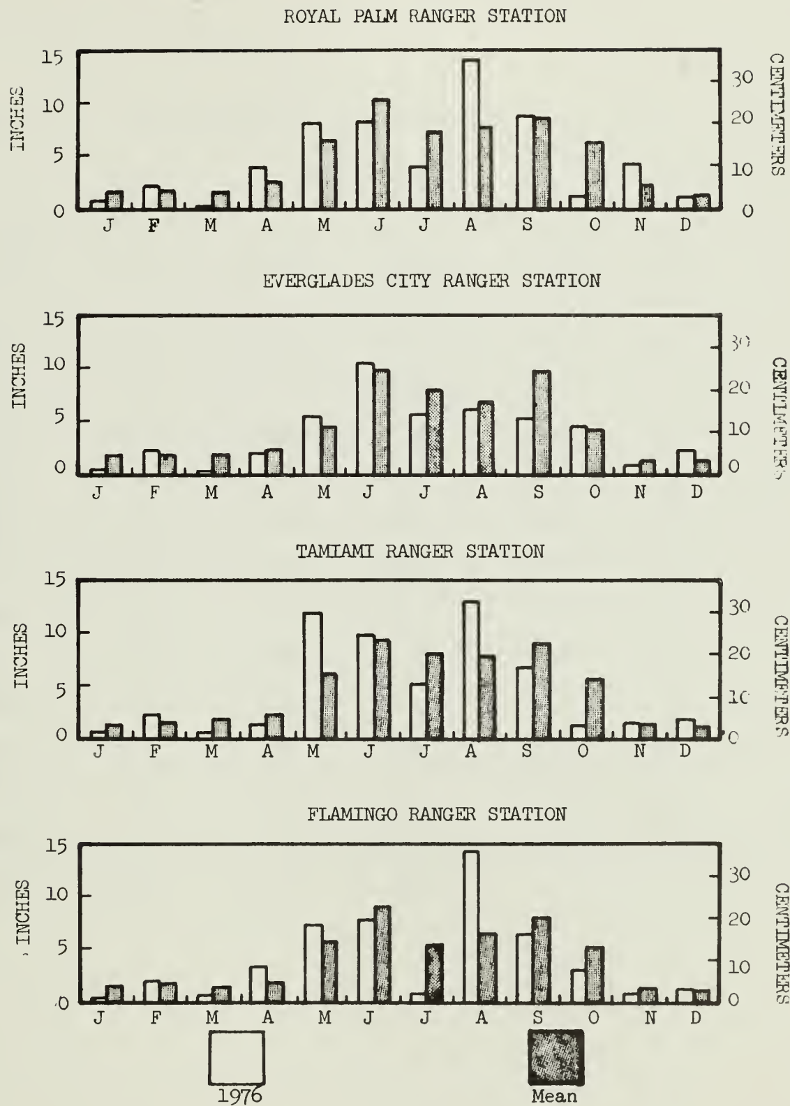
Figure 5 : 1976 Rainfall and Mean by Station
