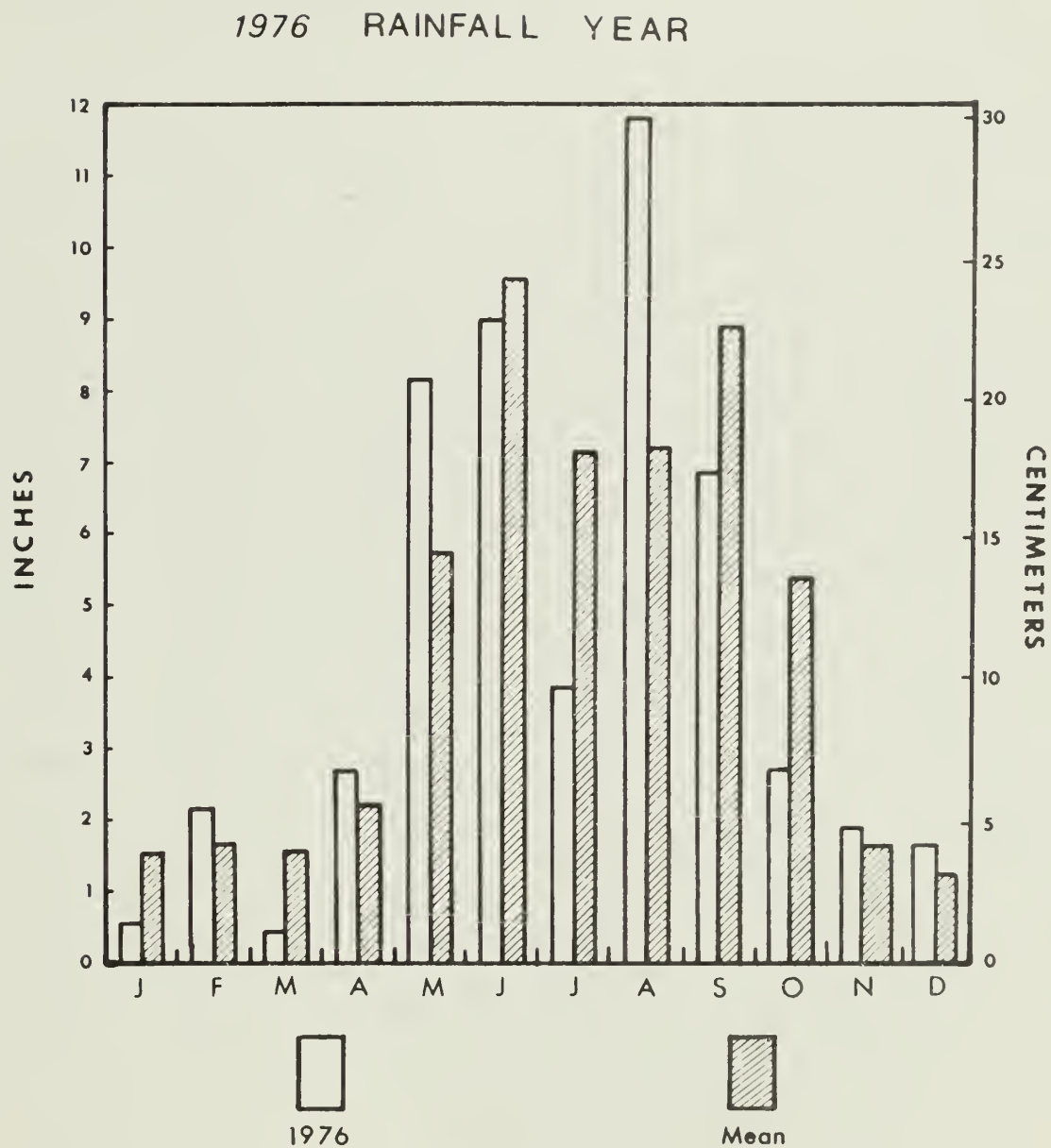
Figure 4: 1976 Rainfall Year, Average of All Four Weather Stations
