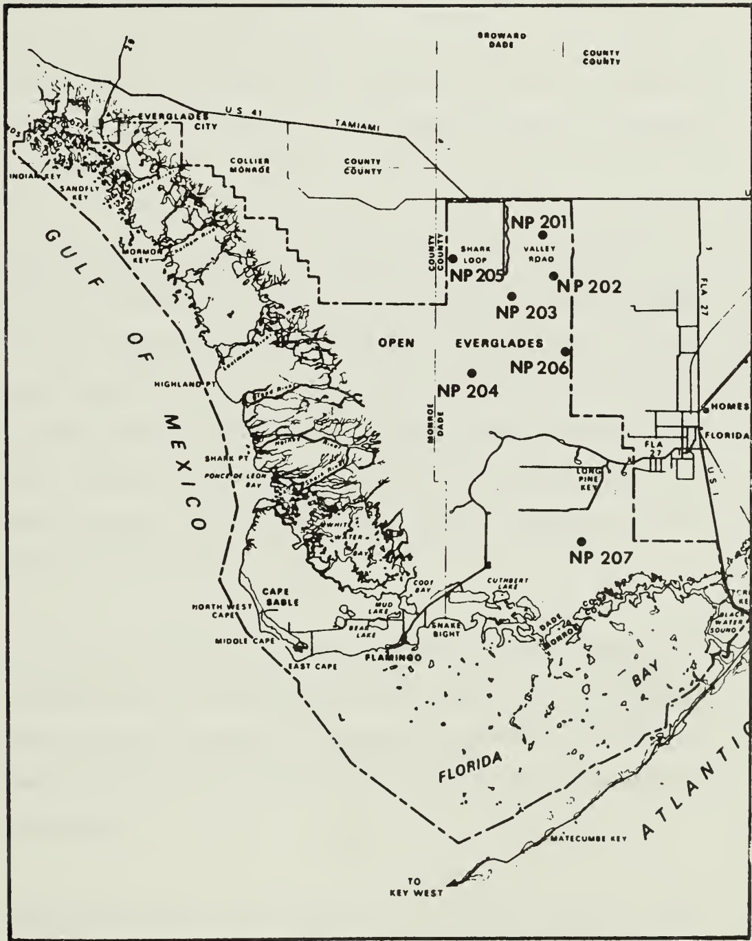
Figure 13: ERTS/LANDSAT Satellite Telemetry Stations, Everglades National Park
