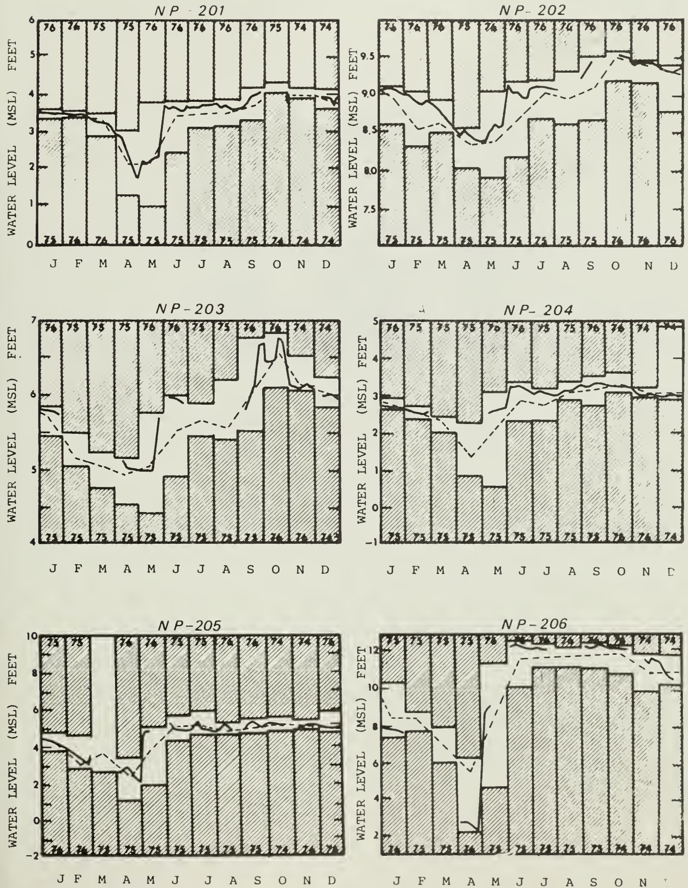
Figure 14: 1976 Hydrographs, ERTS/LANDSAT Satellite Stations
