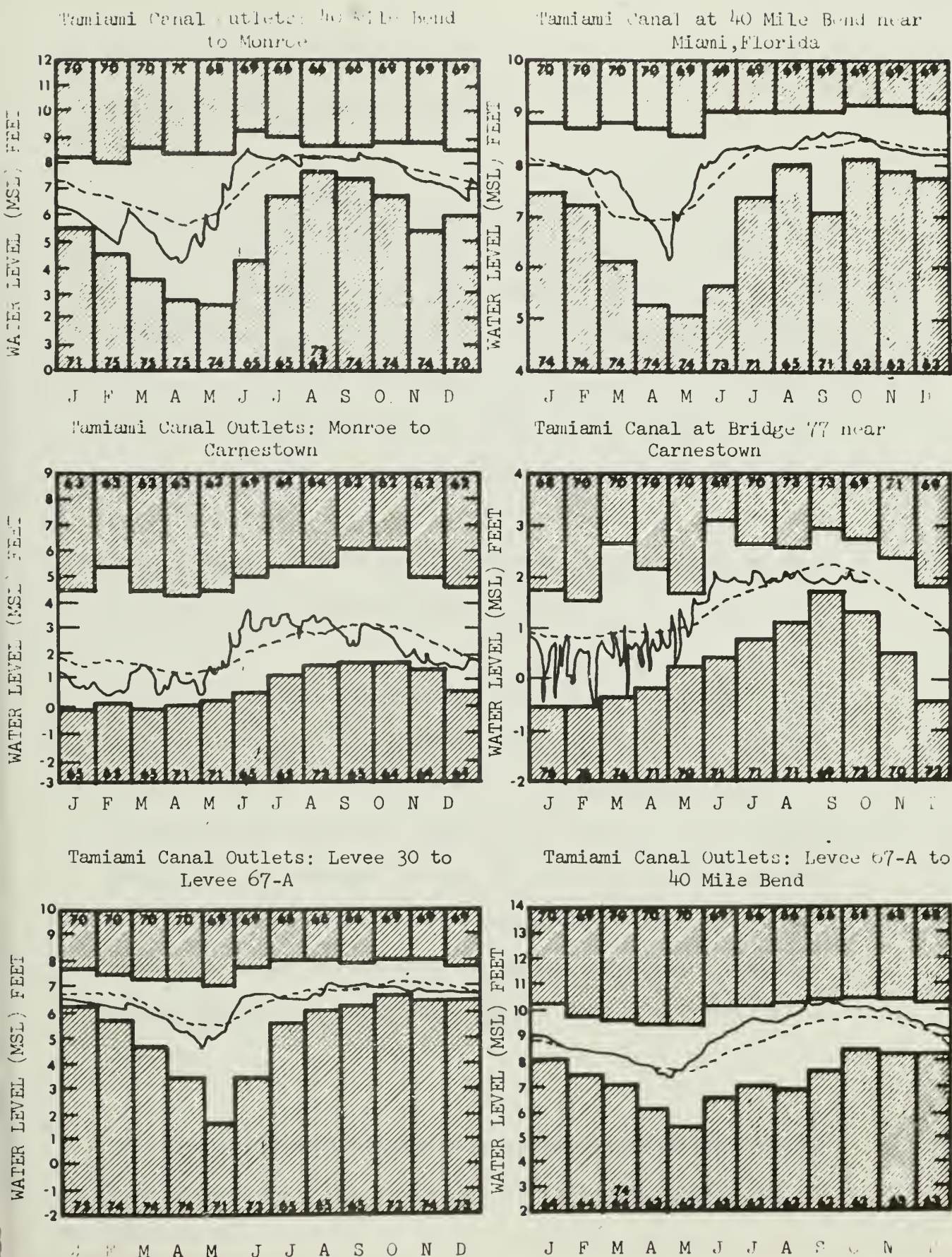
Figure 12: 1976 Hydrographs, Big Cypress Monitoring Stations
