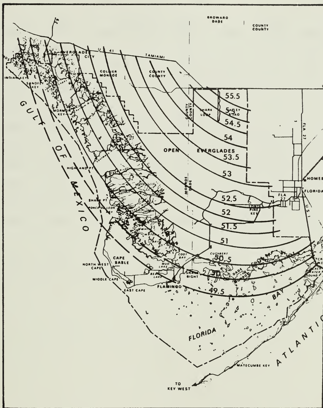
Figure 3: 1976 Mean Rainfall Isohyets, Everglades National Park
