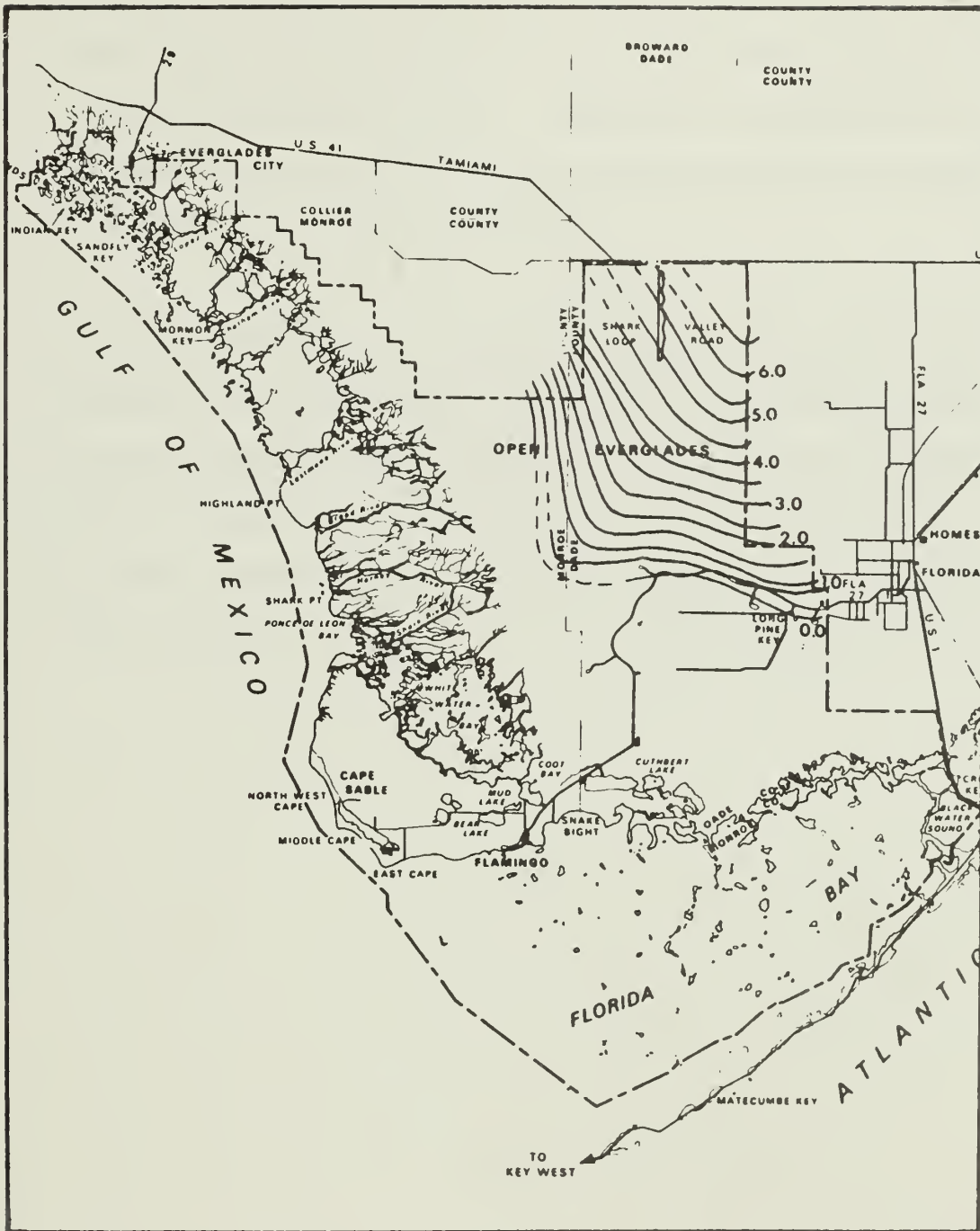
Figure 7: April 1, 1976: Low Water Contours (Contour Interval 0.5 Feet)
