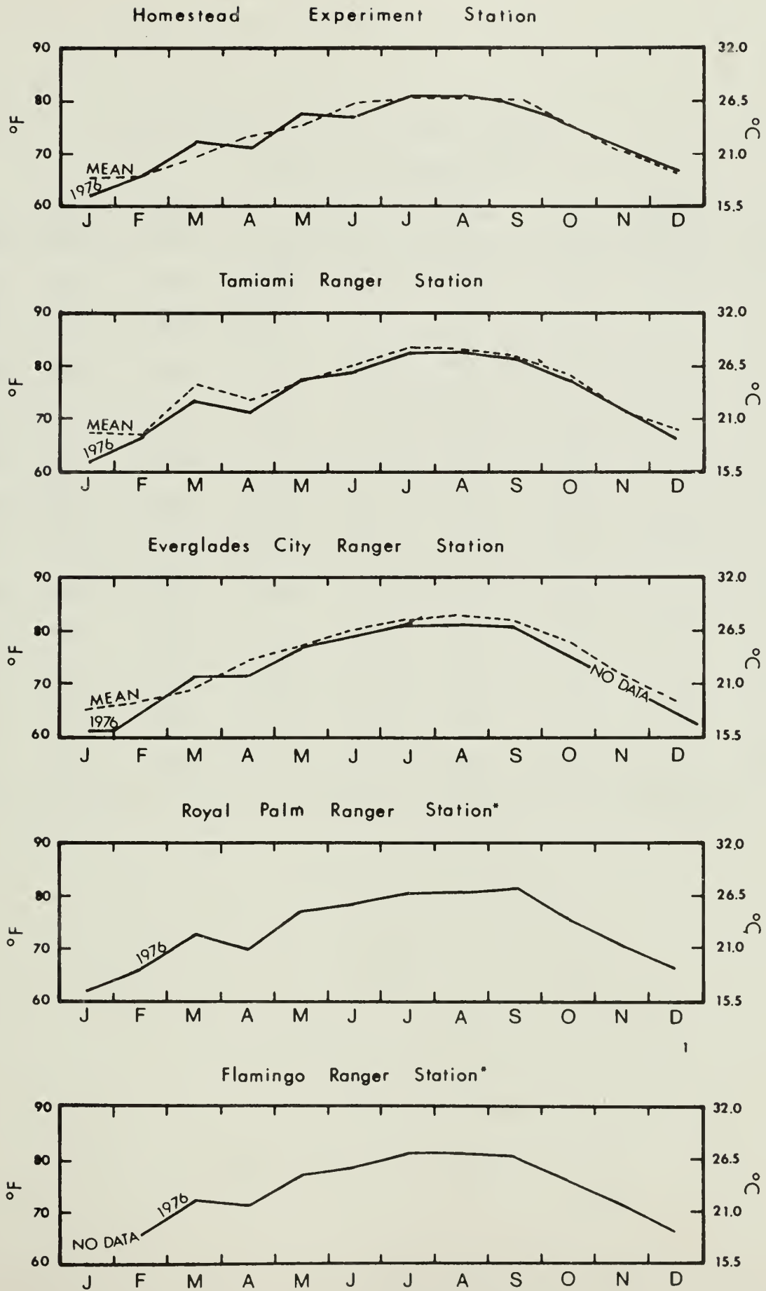
Figure 2: Everglades National Park Temperatures (°F) for 1976
