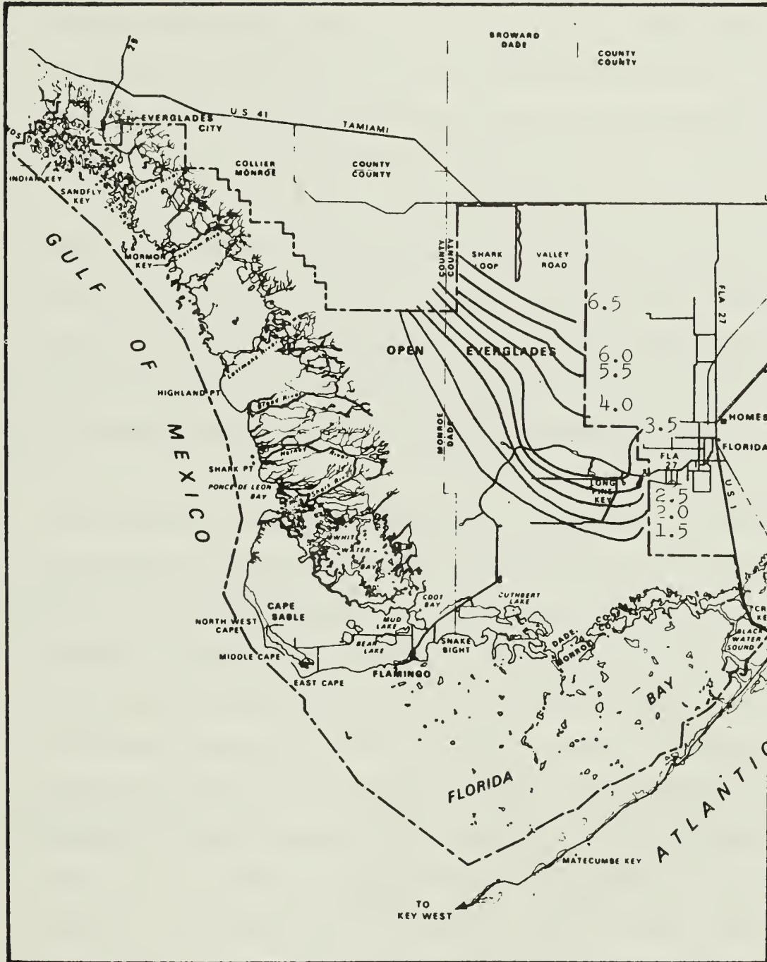
Figure 8. September 20, 1976, High Water Level Contours, Everglades National Park
