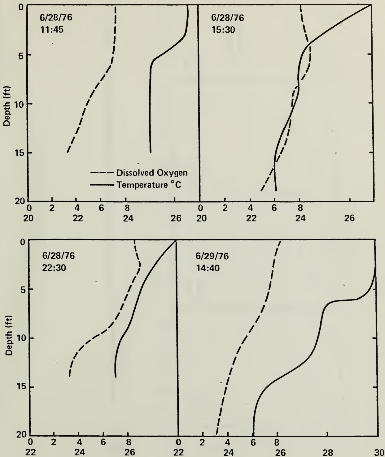
Figure 8 Diurnal Dissolved Oxygen and Temperature Study of Buckhorn Arm
