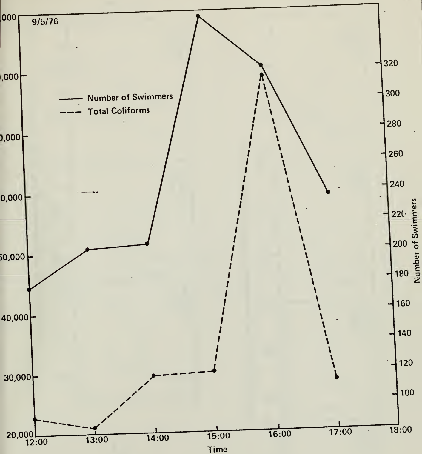
Figure 6 NUMBER OF SWIMMERS vs TOTAL COLIFORM AT TRAVERTINE
