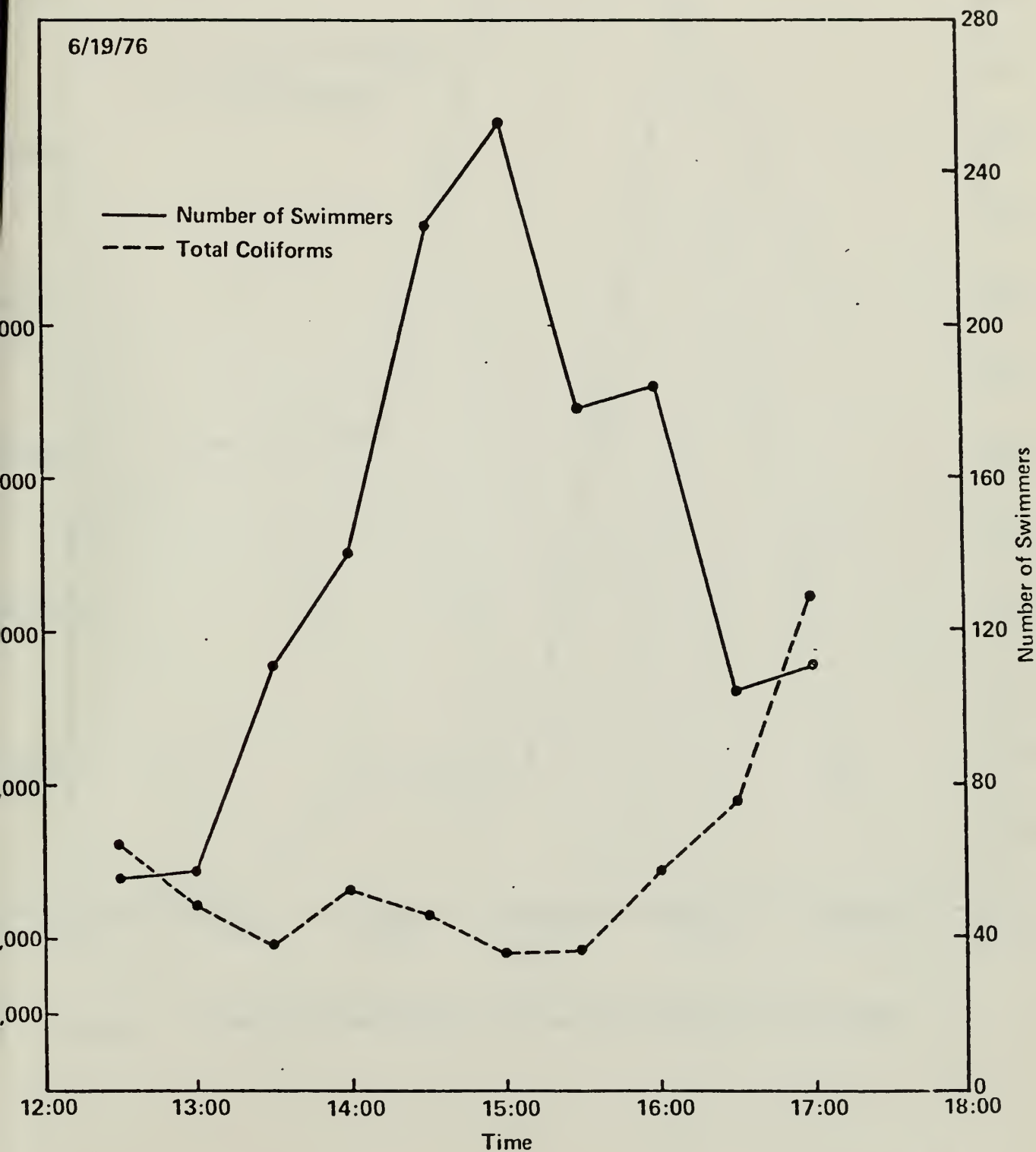
Figure 5 NUMBER OF SWIMMERS vs TOTAL COLIFORM AT TRAVERTINE
