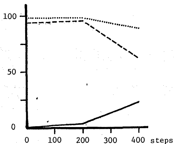
Figure B1. Change in algal cover at Sunset Cliffs with increasing trampling intensity.
