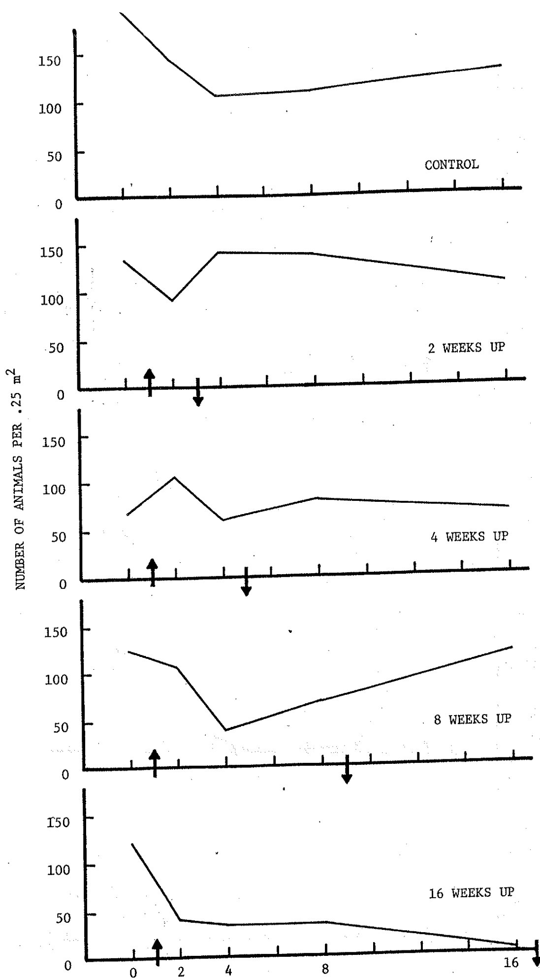
Figure B4. Average density of Phragmatopoma californica .
