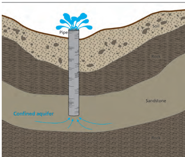
Figure 9. Schematic of an artesian well. Hydraulic pressure in a confined aquifer causes groundwater to rise to a point where hydrostatic equilibrium is reached. An artesian well or artesian flowing spring results if that equilibrium point is above the ground surface. Graphic by Trista Thornberry-Ehrlich (Colorado State University) after a public domain image created by Pearson Scott Foresman and available at http://en.wikipedia.org/wiki/Artesian_aquifer (accessed 6 May 2014).
