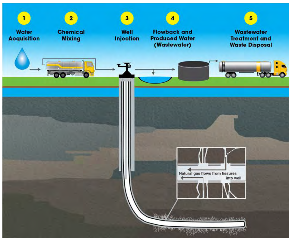
Figure 28. Schematic of hydraulic fracturing (fracking). Horizontal blue line represents an aquifer, which is isolated from the well bore by steel casing and cement. The drill pipe becomes horizontal at approximately 460 m (1,500 ft). Environmental Protection Agency graphic, available at: http://www2.epa.gov/hfstudy/hydraulic-fracturing-water-cycle (accessed 24 April 2015).
