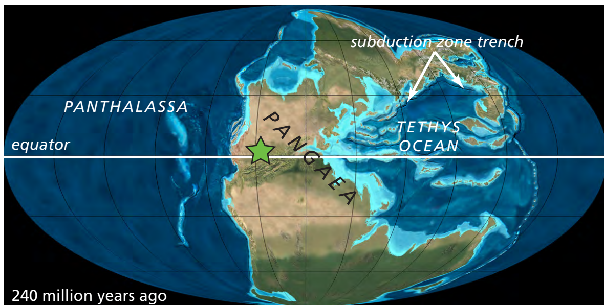
Figure 31. Pangaea. By the Early Triassic Period, all major landmasses had come together to form the supercontinent Pangaea. The C-shaped landmass stretched from pole to pole and surrounded much of the Tethys Ocean. The spine of the "C" was adjacent to a long subduction zone. Much of Earth's surface was covered by a large ocean called Panthalassa. The green star marks the approximate location of Chickasaw National Recreation Area. Annotated by the author. Base paleogeographic map created by Ron Blakey (Colorado Plateau Geosystems, Inc.), available at http://cpgeosystems.com/index.html (accessed 7 May 2014).
