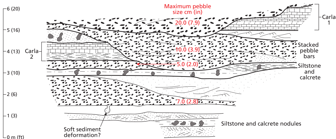
Figure 17. Sketch of the Vanoss Formation near the top of Bromide Hill. The vertical scale is exaggerated approximately three times. The cross-section illustrates the complex relationship between rock type and process. The “Carla” is a lacustrine limestone. The “stacked pebble bars” unit is younger than the limestone, siltstone, and calcrete into which it has incised. Diagram redrafted by Trista Thornberry-Ehrlich (Colorado State University) after Donovan and Butaud (1993, figure 10).
