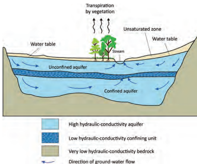
Figure 7. Schematic of an aquifer. Water percolating through the unsaturated zone of unconsolidated sediments or porous rock forms an unconfined aquifer. If a rock layer does not have sufficient porosity or permeability, it forms a barrier to groundwater flow. Groundwater below this confining layer becomes part of a confined aquifer. The Arbuckle-Simpson aquifer has properties resembling both a confined and unconfined aquifer. Hydraulic conductivity is a measure of how easily groundwater flows through pore spaces in the rock unit. Diagram by Hans Hillewaert (Creative Commons Attribution-Share Alike 3.0 Unported license), available online at http://en.wikipedia.org/wiki/Aquifer (accessed 6 May 2014).
