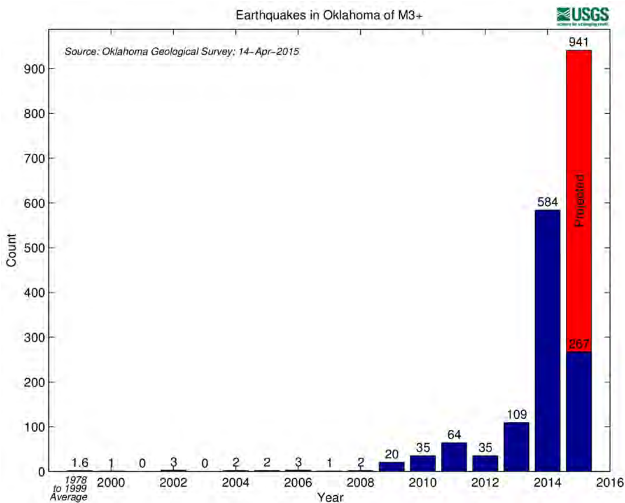
Figure 29. Oklahoma earthquakes of magnitude 3.0 and greater, 1978 to April 14, 2015. Since October 2013, earthquakes in Oklahoma have increased significantly. Wastewater from hydrocarbon production that is injected into the subsurface contributes to these earthquakes. Graph from US Geological Survey, available at http://earthquake.usgs.gov/earthquakes/states/?region=Oklahoma (accessed 31 July 2015).
