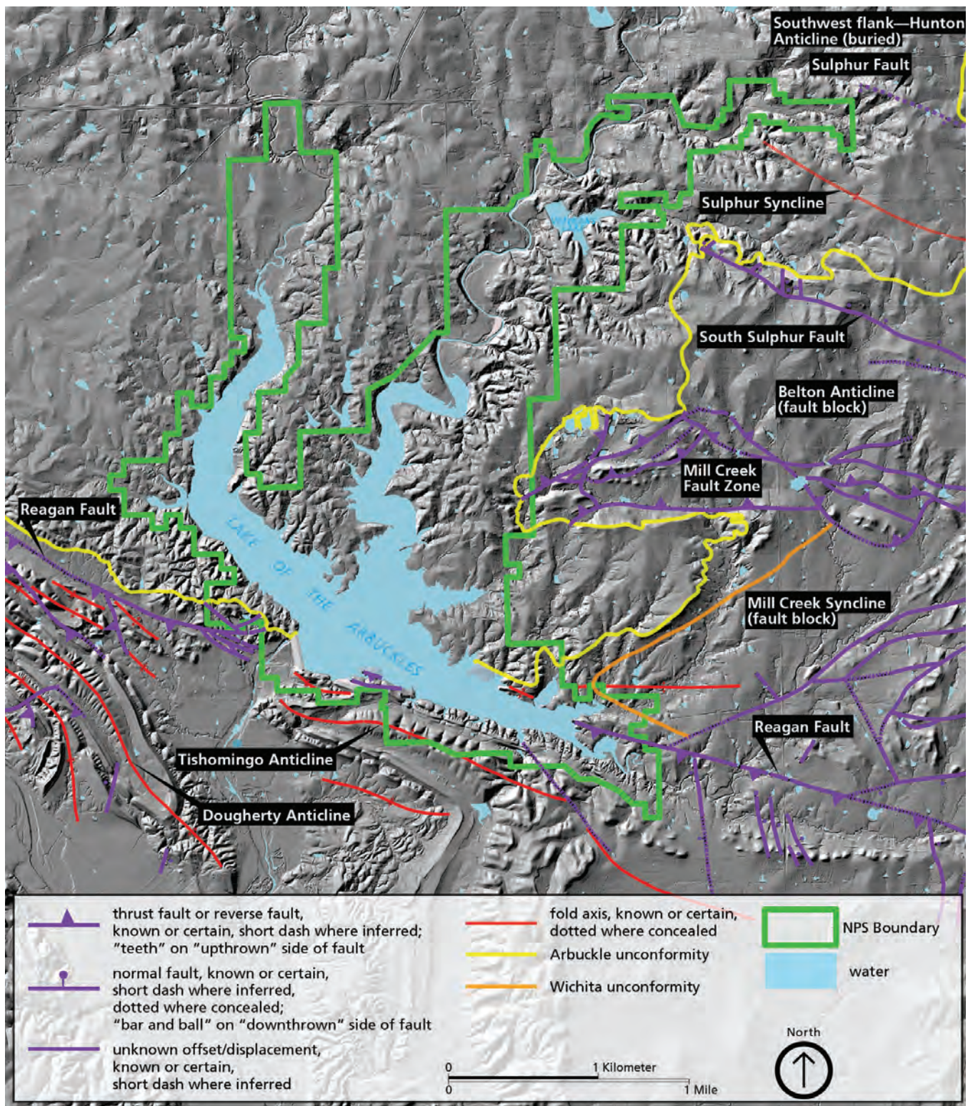
Figure 19. Map showing the structural features and related Pennsylvanian angular unconformities in and near Chickasaw National Recreation Area. Graphic by Trista Thornberry-Ehrlich (Colorado State University) after Blome et al. (2013, figure 6), using GRI GIS data.
