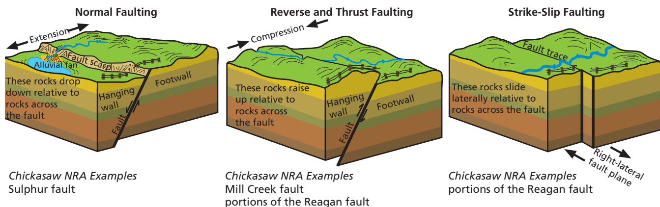
Figure 18. Schematic illustrations of three general fault types. In a fault, movement occurs along a fault plane. “Footwalls” are below the fault plane and “hanging walls” are above it. In a normal fault, crustal extension (pulling apart) moves the hanging wall down relative to the footwall. In a reverse fault, crustal compression moves the hanging wall up relative to the footwall. A thrust fault is similar to a reverse fault, but has a dip angle of less than 45 degrees. In a strike-slip fault, the relative direction of movement of the opposing plate is lateral. When movement across the fault is to the right, it is a right-lateral (dextral) fault, as illustrated above. When movement is to the left, it is a left-lateral (sinistral) fault. All three types are present in the Arbuckle Mountains; the Sulphur fault is a normal fault, Mill Creek fault is a reverse fault and movement along the Reagan fault incorporates both reverse and strike-slip motion. Graphic by Trista Thornberry-Ehrlich (Colorado State University).
