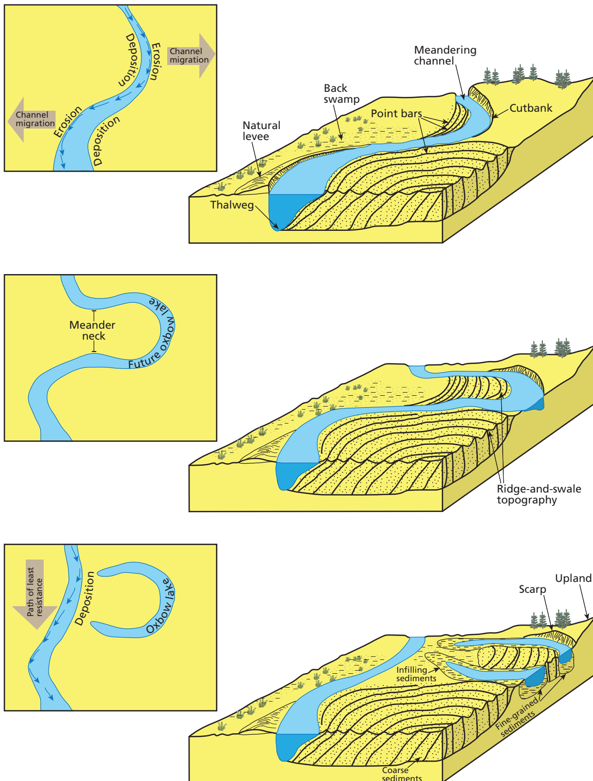
Figure 24. Schematic of the features common to a meandering river. Point bars are areas of deposition. Lateral erosion takes place at cutbanks. The thalweg is the path of greatest current velocity, represented by blue arrows within the stream. When a meander neck is cut off, an oxbow lake forms. Time progression is from upper graphic to lower graphic. Graphic by Trista Thornberry-Ehrlich (Colorado State University).
