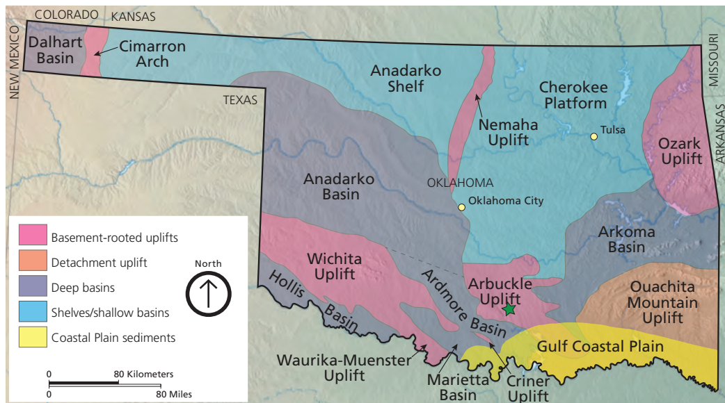
Figure 4. Geologic provinces of Oklahoma. Chickasaw National Recreation Area (green star) lies within the Arbuckle Uplift, which contains some of the thickest accumulations of Paleozoic sedimentary rock in the central United States. Map by Trista Thornberry-Ehrlich (Colorado State University) after an Oklahoma Geological Survey diagram, available at http://www.ogs.ou.edu/MapsBasic/Provinces.jpg (accessed 4 March 2014) and comments from Neil Suneson (Oklahoma Geological Survey, written communication, 24 November 2014). Basemap by Tom Patterson (National Park Service), available at http://www.shadedrelief.com/physical/index.html (accessed 15 October 2014).
