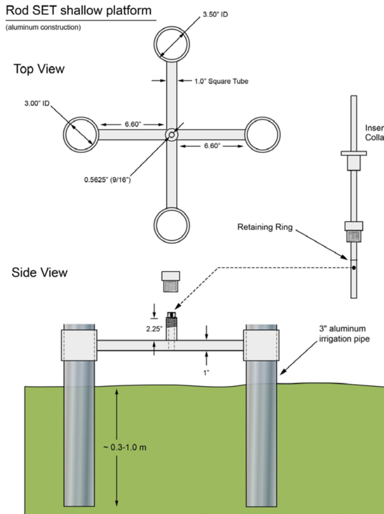
Figure 3.29. Shallow RSET mark (Callaway et al. 2013).
