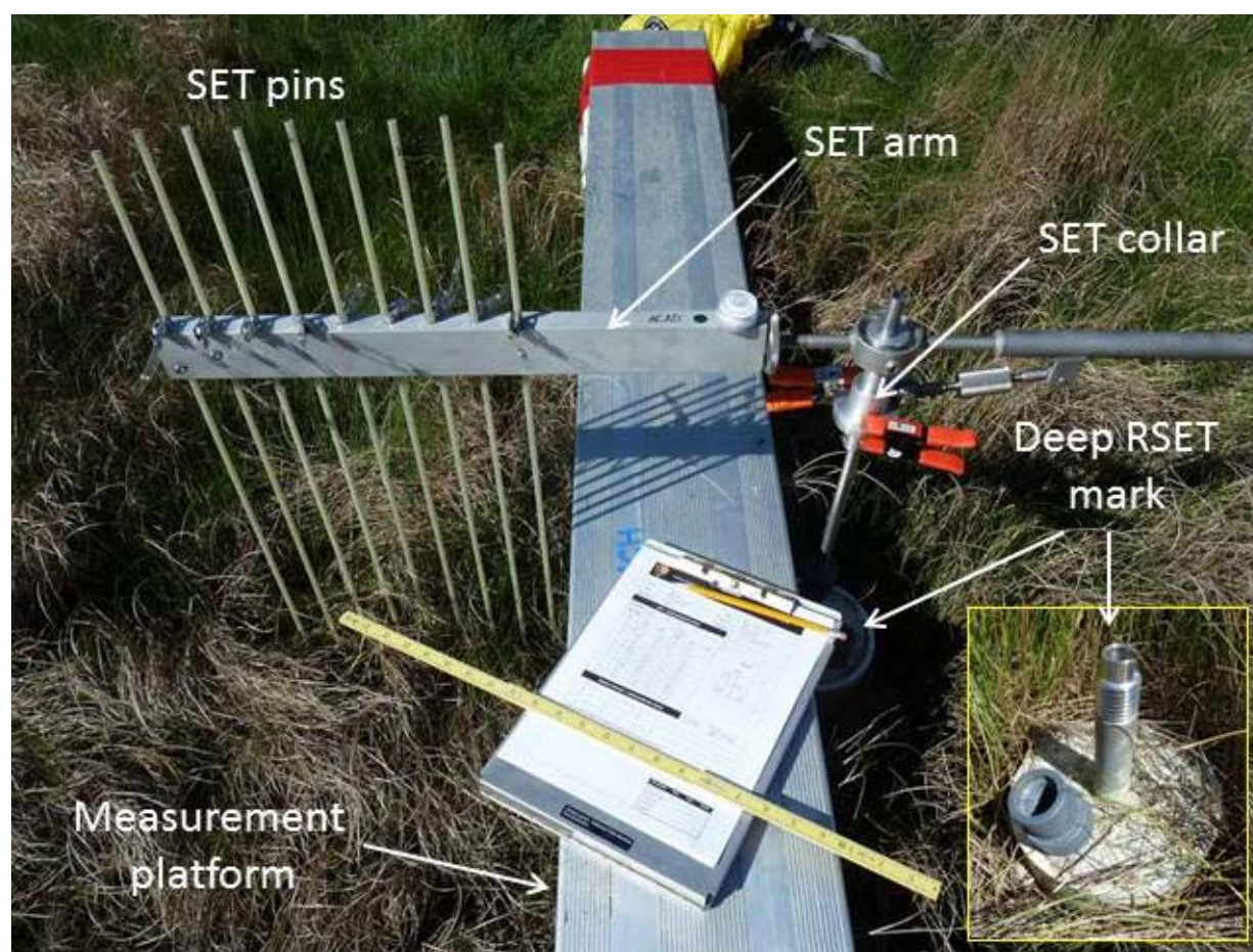
Figure 3. Rod SET instrument deployed in a tidal salt marsh (Acadia National Park, Maine). The instrument attaches to the deep RSET mark and the SET arm is extended over the marsh surface at fixed directions. The arm is carefully plumbed so it is horizontal, and each of nine pins is lowered until it makes contact with the wetland surface. The height of each pin remaining above the arm is measured to the nearest millimeter at every sampling. Change is recorded as the change in height of each pin over time. Four positions provide 36 pin readings covering an area of approximately 1.5m 2 .
