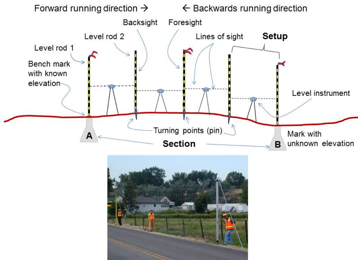
Figure 6.16. Schematic showing basic concepts involved with leveling. The elevation is transferred from a bench mark (with known elevation) to a mark whose elevation is unknown. This transfer is accomplished by measuring the height difference between the two marks. Temporary points (turning points) are used to hold an elevation as the level moves from Point A to Point B and then back again.
