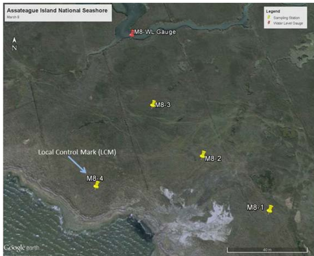
Figure 6.2. Map showing locations of four SET stations: M8-1 through M8-4. Map also shows location of a local water level recorder (M8-WL Gauge). Only one SET station will be chosen as the local control mark (LCM), in this example, M8-4.
